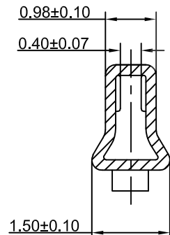
Section C-C
