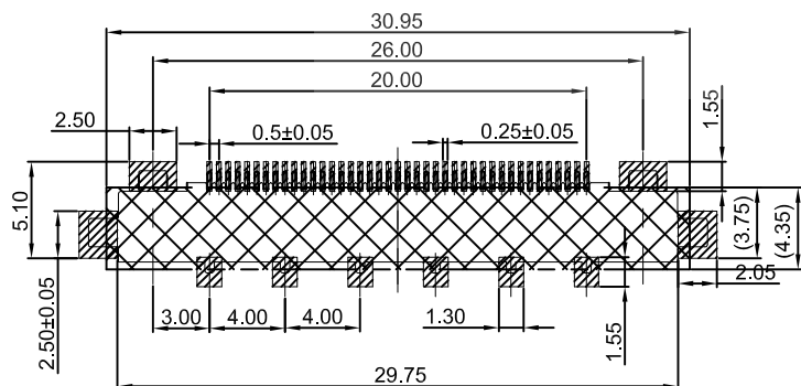
APPLICABLE P.C.B DIMENSION
