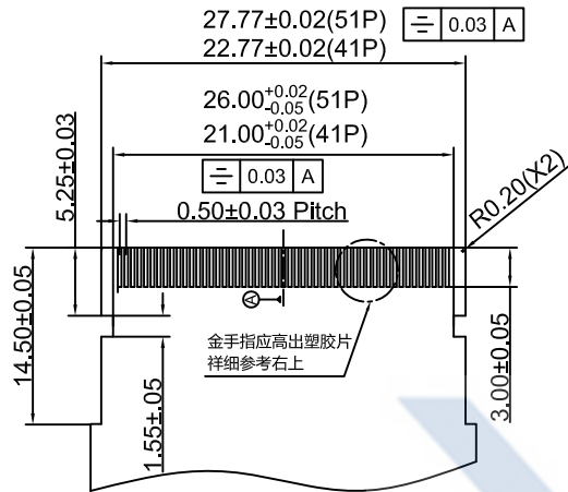
Drawing of FFC Cable Tailer
